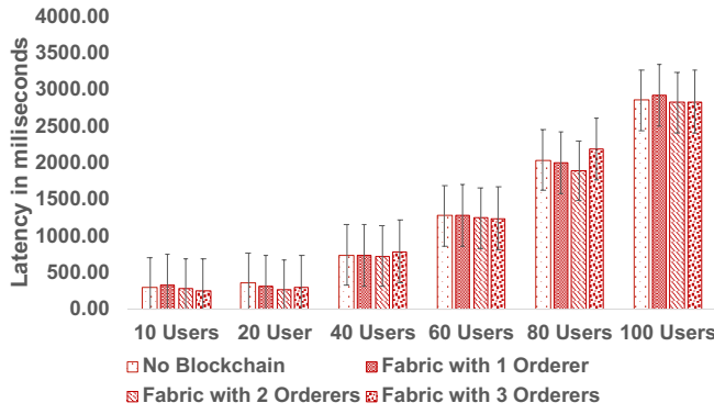
(a) Latency vs Load
