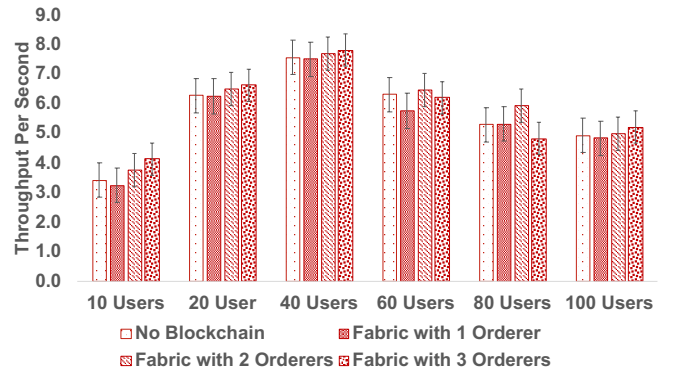
(b) Throughput vs Load
