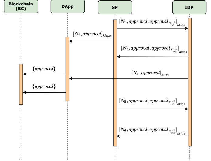
Fig. 2: Protocol flow of adding an entity
